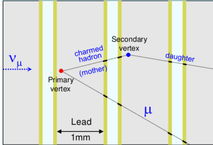
Figure 3.2: Charmed hadron decay in \nu_\mu CC interaction
