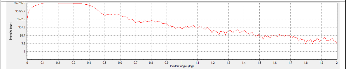
Figure No. 24 - X-ray reflectivity Gd(6nm)
