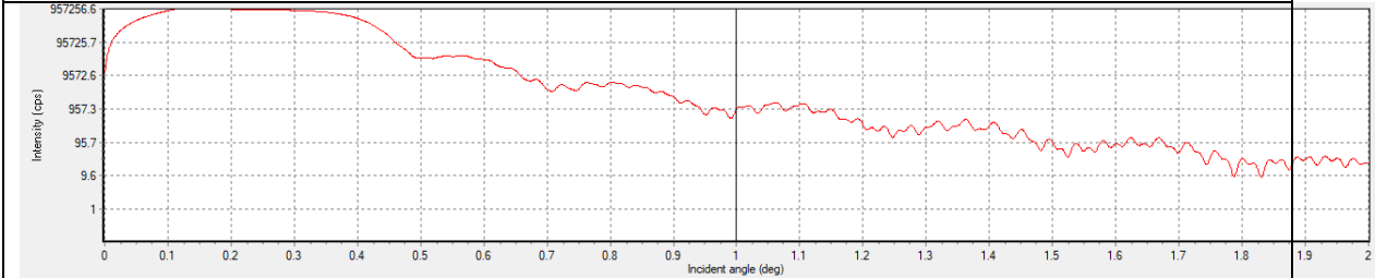
Figure No. 25 - X-ray reflectivity Gd(12nm)
