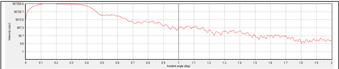
Figure No. 23 - X-ray reflectivity Gd(3nm)
